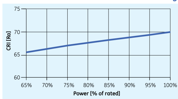
StreetWise™ dimmed colour rendering
